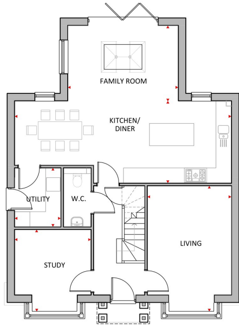
PLOT 6 GROUND FLOOR
